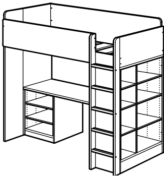
Total size: 197×99×207 cm (for mattress size: 90×200 cm). (090.319.07)
